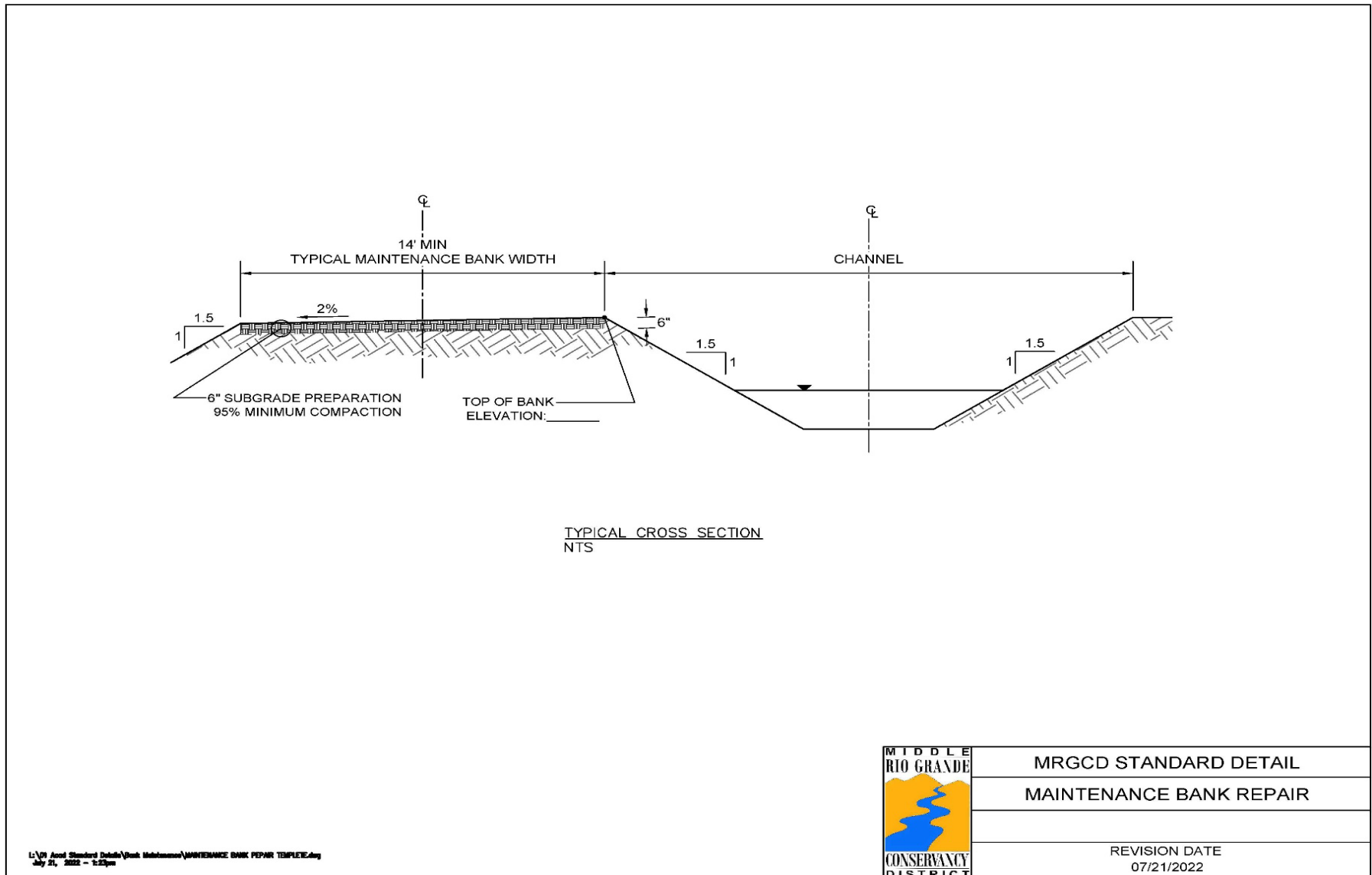
Figure 6: MRGCD Standard Detail for Maintenance Bank Repair
